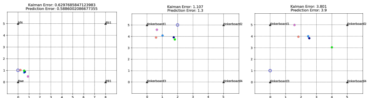
Figure 40: Sample Results of Localization Experiments. Left: Experiment 1 on Position (0,1). Middle: Experiment 2 at Position (2,5). Right: Sample of Step 1 of Experiment 2
