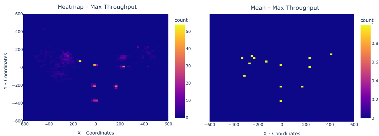
Figure 57: Heat Map of Max (Left) and Mean (Right) Throughput
