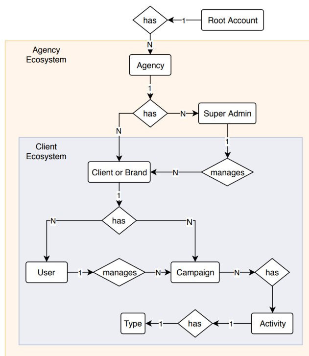
Figure 31: Stakeholders ER Diagram
