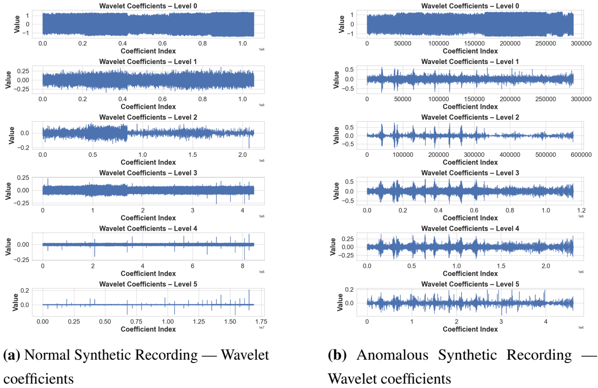
Figure 5.8: Comparison of Anomalous and Normal Recordings Wavelet Coefficients
