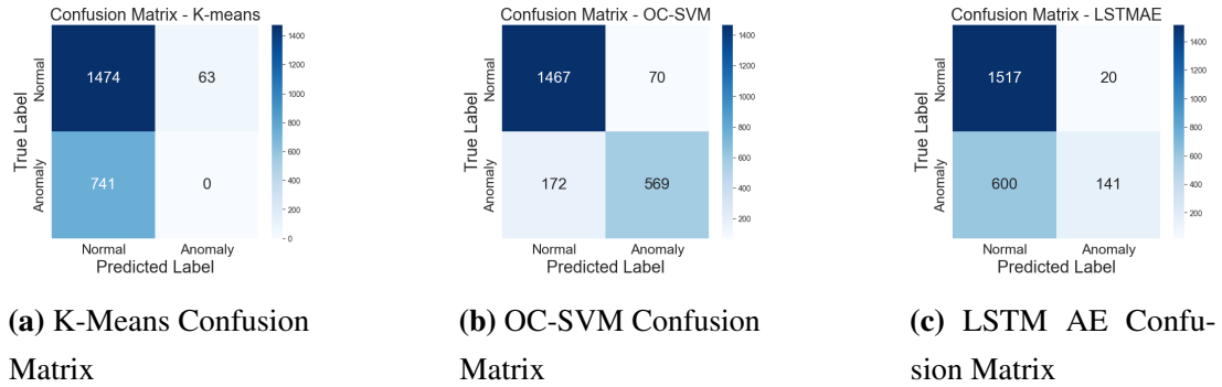
Figure B.1: Comparison of Confusion Matrices for Washing Machine Dataset
