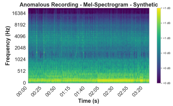
(b) Anomalous Synthetic Recording — Mel-Spectrogram
