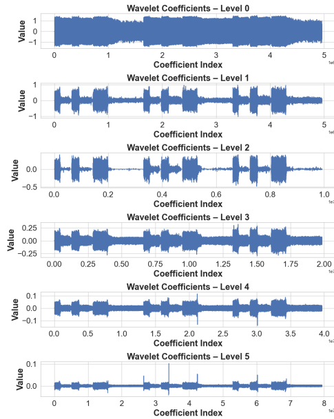
(a) Normal Real Recording — Wavelet coefficients
