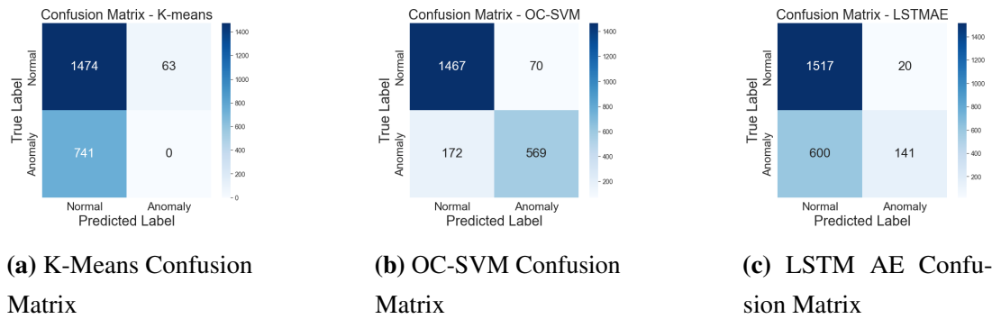
Figure 5.13: Comparison of Confusion Matrices for Washing Machine Dataset
