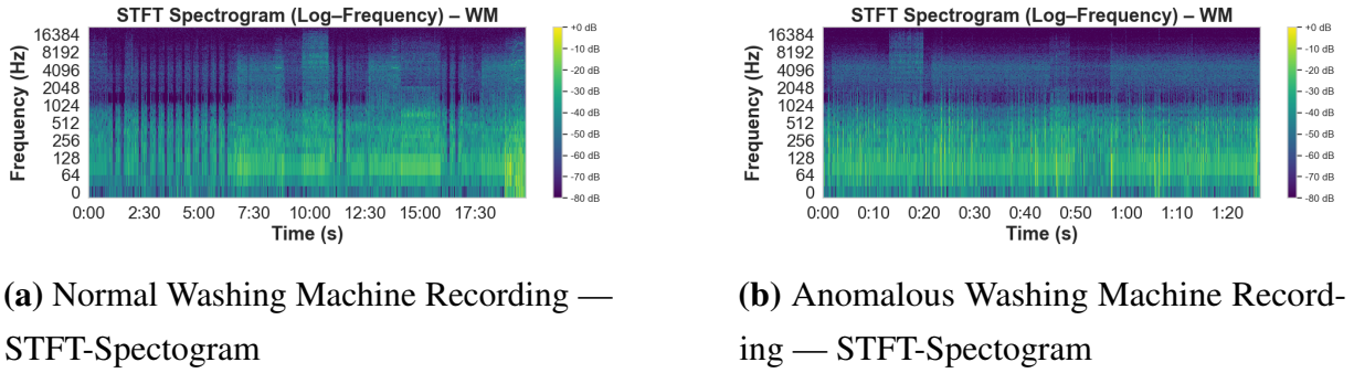
Figure 5.3: Comparison of Anomalous and Normal Recordings STFT-Spectrograms
