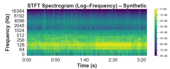
(b) Anomalous Synthetic Recording — STFT Mel-spectrogram
