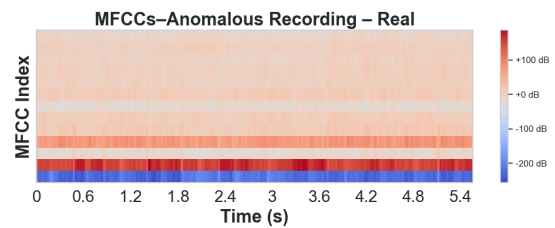
(b) Anomalous Real Recording — MFCCs
