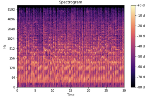
Figure 2.1: Mel-spectrogram [80]
