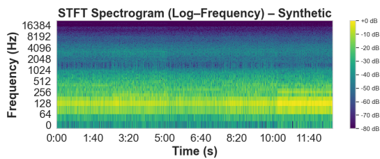
(a) Normal Synthetic Recording — STFT Mel-spectrogram
