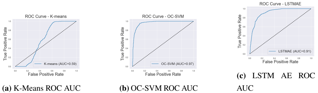
Figure B.2: Comparison of ROC AUCs for Washing Machine Dataset
