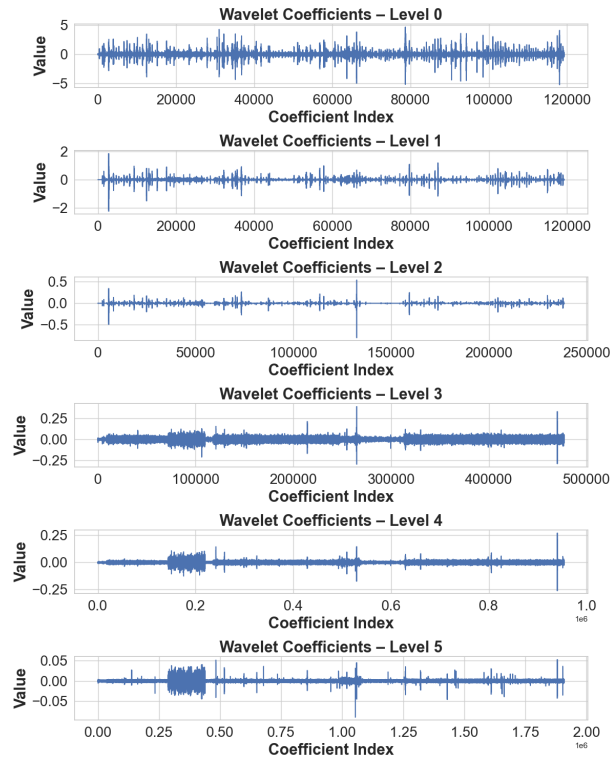
(b) Anomalous WM Recording — Wavelet coefficients
