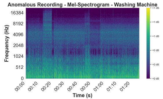
(b) Anomalous Washing Machine Recording — Mel-Spectrogram
