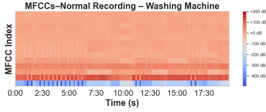
(a) Normal WM Recording — MFCCs
