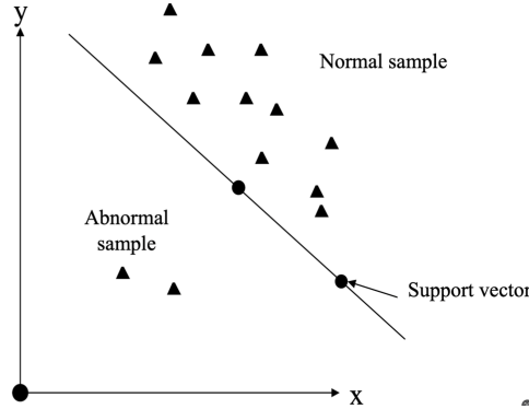
Figure 2.3: OC-SVM Diagram [42]
